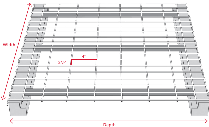
STEP CHANNEL
