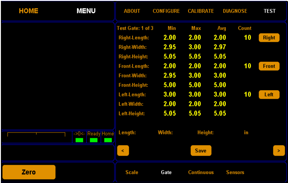
Figure 78 First Gate Test Screen
